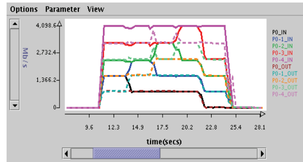
Figure 8. Basic IPv4 router throughput demonstration showing input rates (solid) and output rates (dashed)
